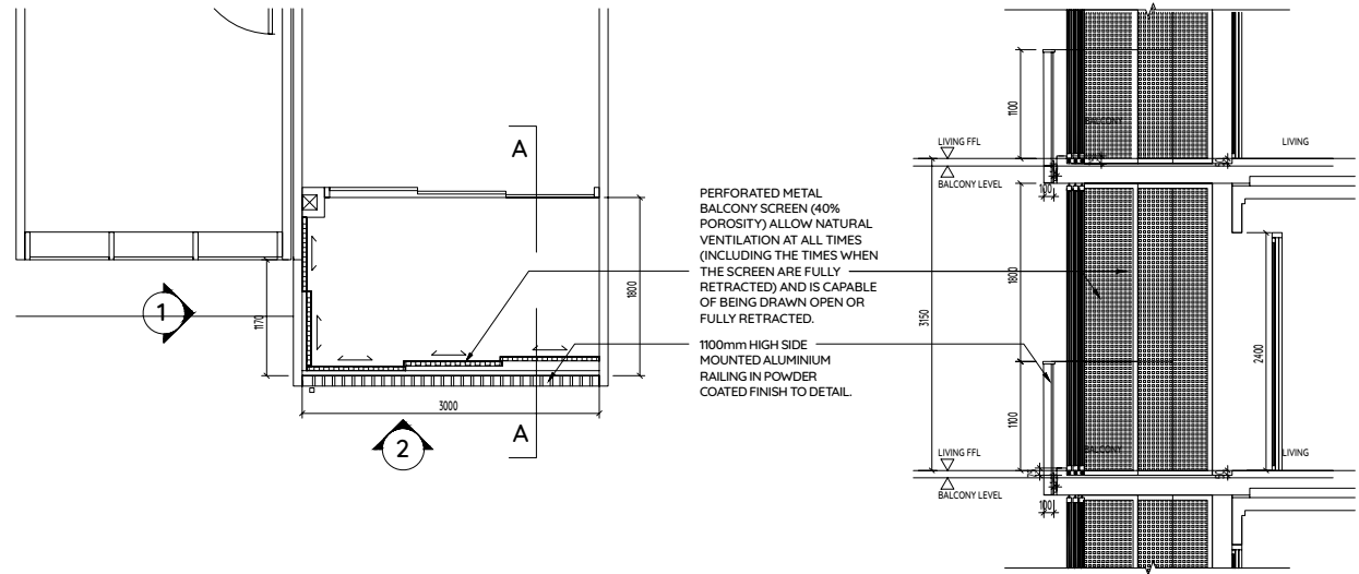
TYPICAL BALCONY SCREEN (CLOSED) - PLAN
