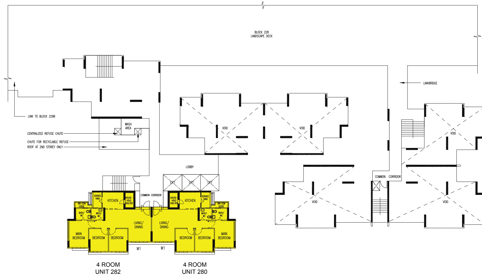
BLOCK 229A (2ND STOREY FLOOR PLAN)
