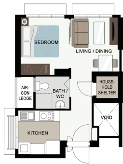
LAYOUT IDEAS FOR 2-ROOM FLEXI (TYPE 1) APPROX. FLOOR AREA 38 sqm (Inclusive of Internal Floor Area of 36 sqm and Air-con Ledge)
